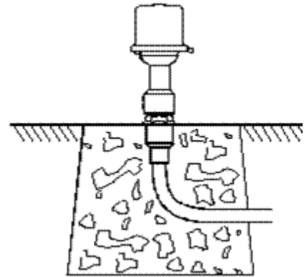
FIGURE 2 – INSTALLATION ON A CURVE TUBE
