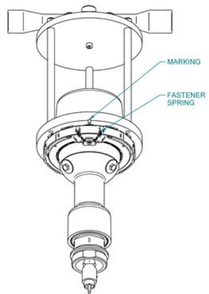
FIGURE 3 – LEVELLING
