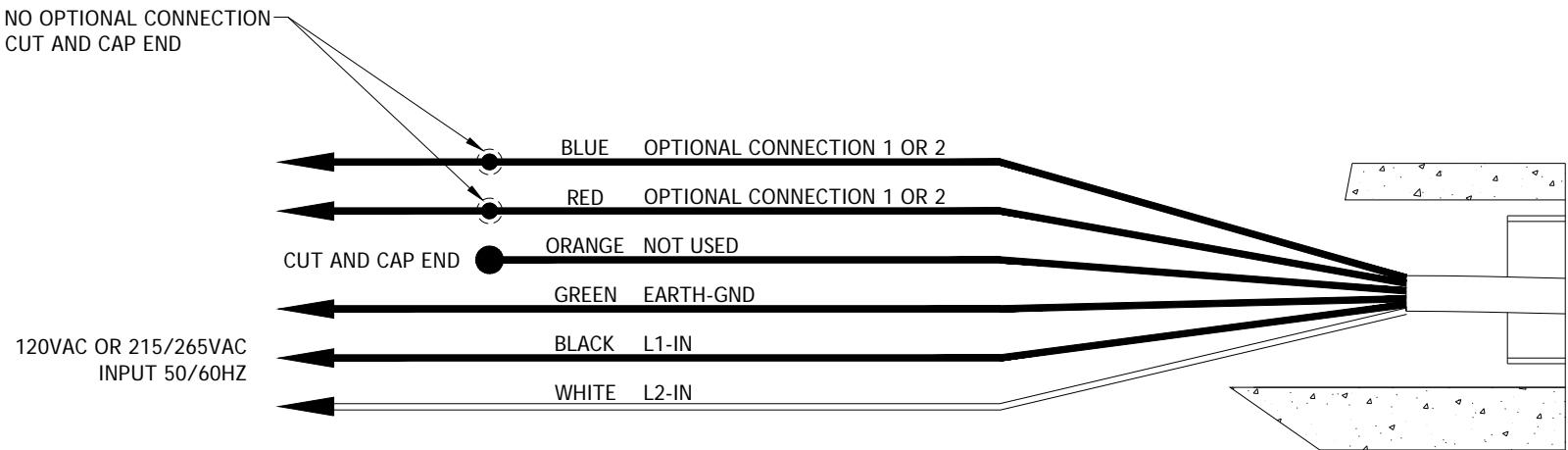
DETAIL A: SYSTEM WIRE SPLICING
