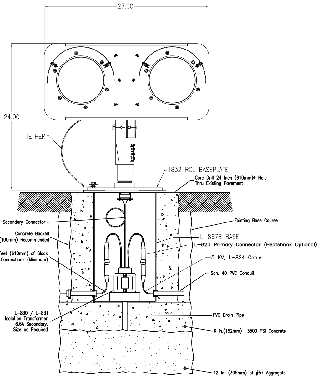
EXAMPLE OF BASE MOUNTED L-804 FIXTURE INSTALLATION IN EXISTING SHOULDER SECTION CURRENT DRIVEN (UNMONITORED)
