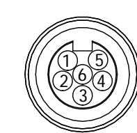
SECTION A-A: PLUG P1 (TYP ALL PLUG CORDSETS)
