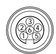
SECTION B-B: RECEPTACLE R1 (TYP ALL RECEPTACLE CORDSETS)
