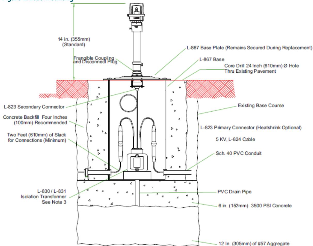
Figure 1: Base Mounting
