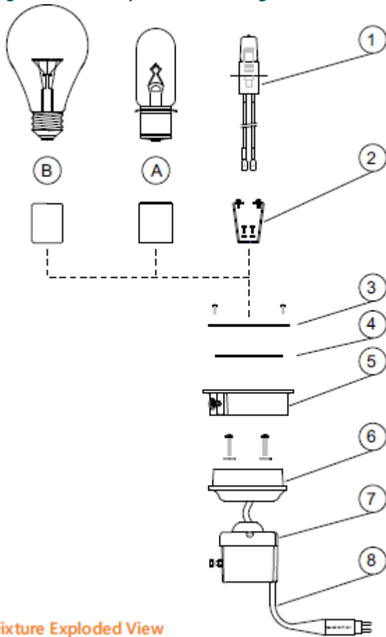
Figure 5: MIRL Exploded Parts Diagram
