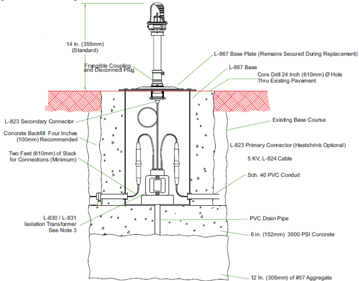
Figure 2: Base Mounting
