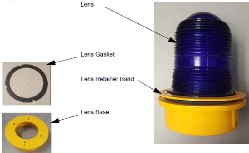
Figure 3: Lens Assembly
