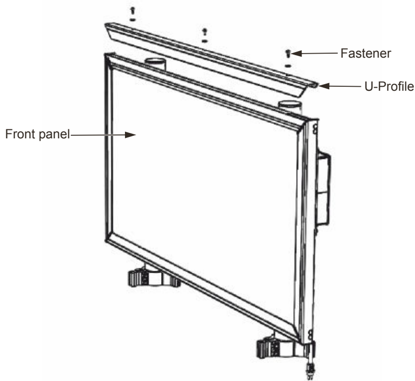
Figure 21: Front panel overview
