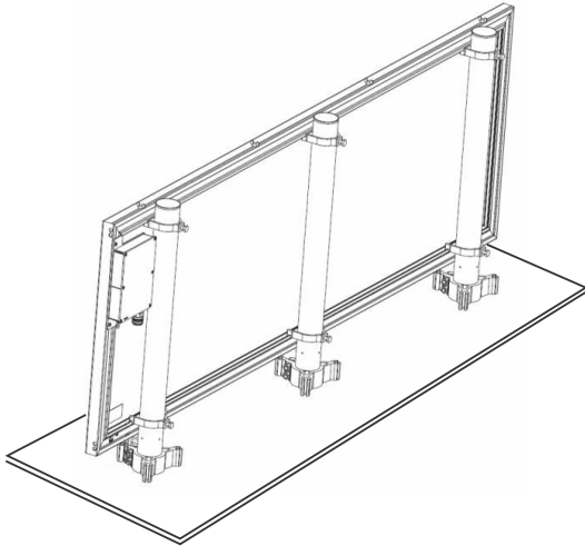
Figure 38: Correct assembly of sign
