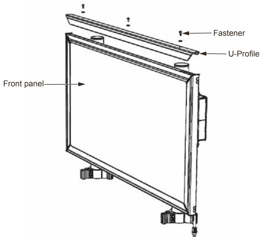
Figure 20: Front panel overview
