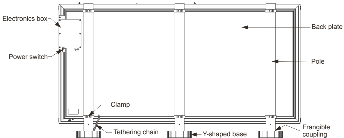
Figure 35: SafeLED sign back
