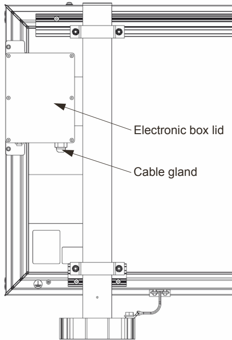
Figure 29: Electronic box overview
