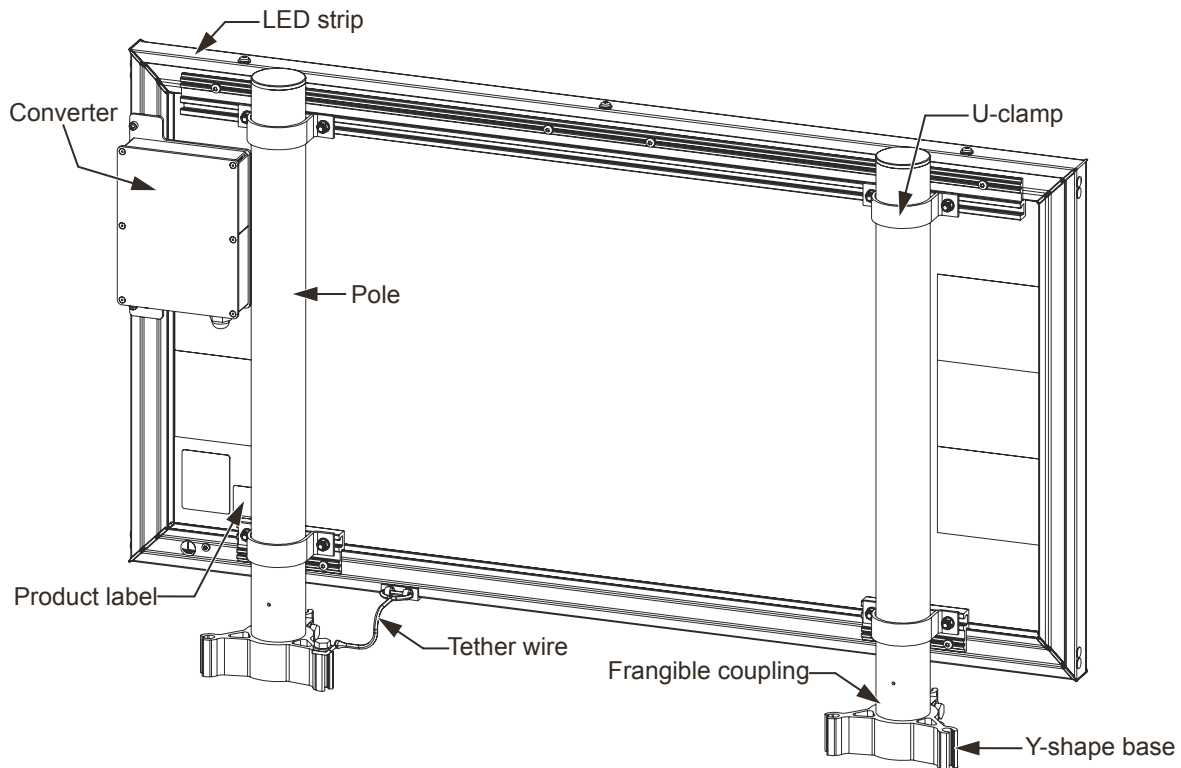
Figure 33: Sign back
