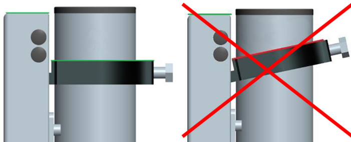
Figure 37: To the left a correct installation of a clamp
