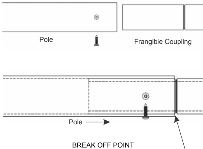
Figure 32: Frangible coupling overview
