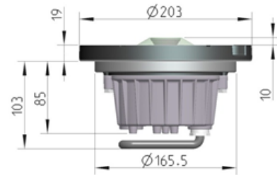
SafeLED TE-I-230V side view
