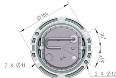
SafeLED TE-I-230V top view
