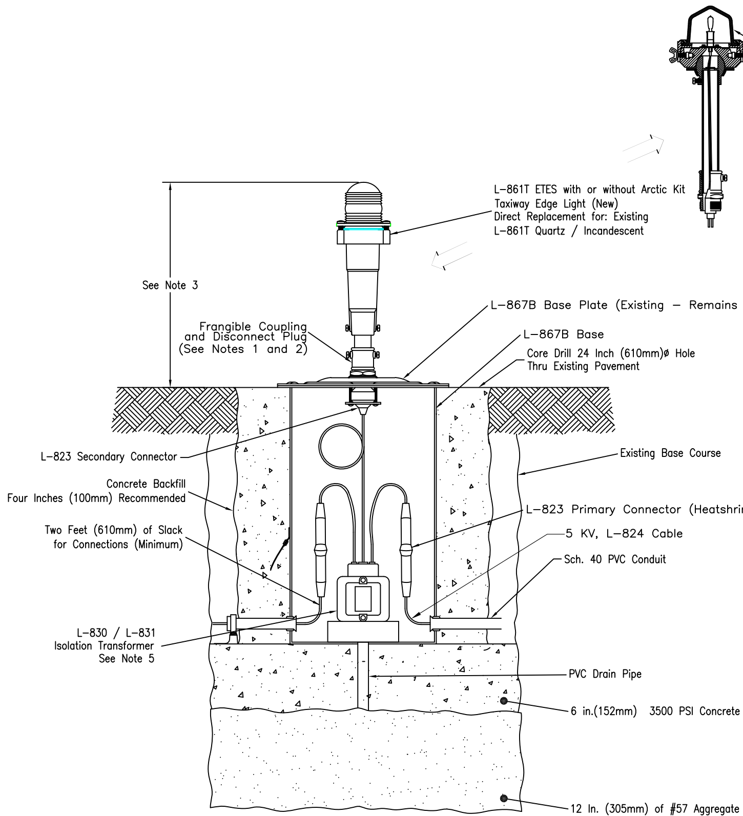
EXAMPLE OF BASE MOUNTED L-861T FIXTURE INSTALLATION IN EXISTING SHOULDER SECTION
