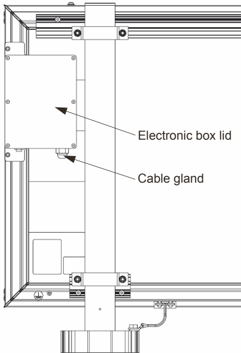
Figure 39: Electronic box overview
