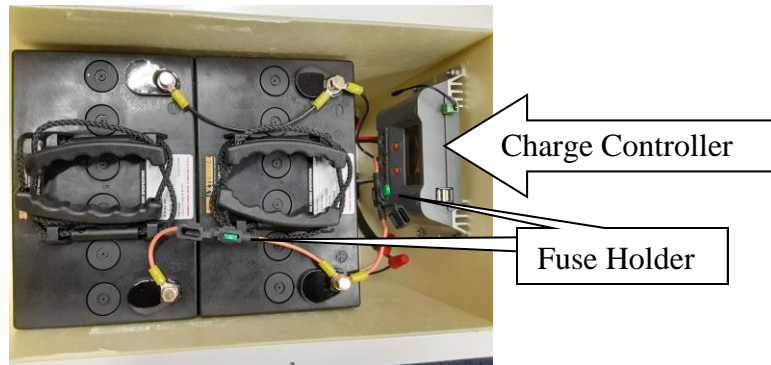
Figure 7. Fuse Installation
