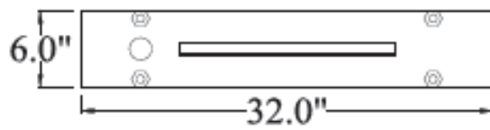
Anchor Assembly Top View
