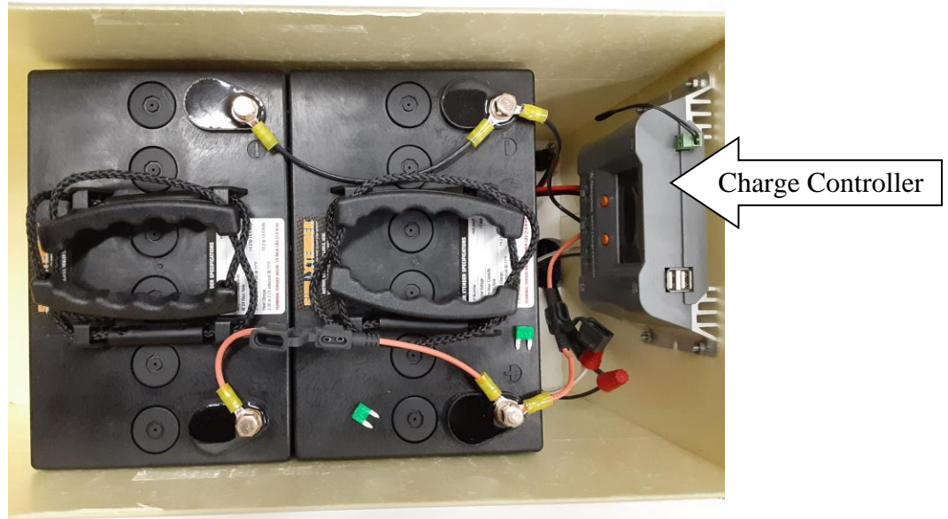
Figure 12. Charge Controller
